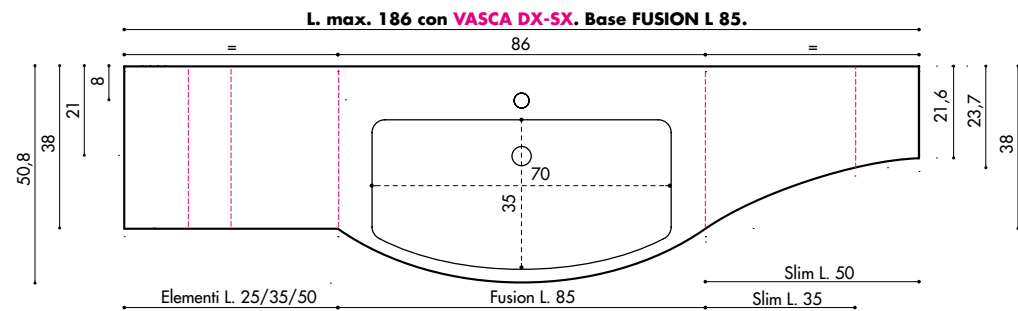
Art. F002 Per basi portalavabo Fusion L 85 cm P. 280
