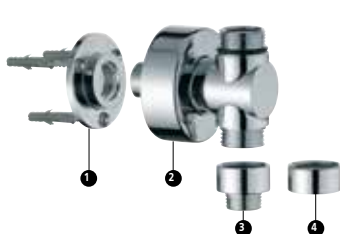
330 RA € 102,30 Water punch outlet and wall bearing for shower columns, multifunction: - high wall bearing - high punch for water outlet - low punch for water outlet with closing plug - low punch for outlet water, for shower flexible hose
